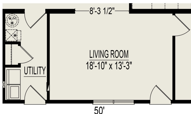
CRAWLSPACE PLAN
